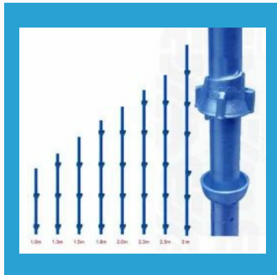
Cuplock Standard .
