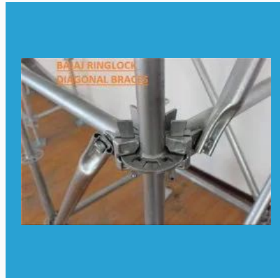
Ringlock Diagonal Bracings
