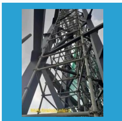
Ringlock Ledger .
