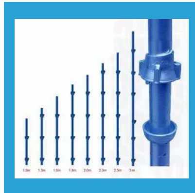
Cuplock Standard
